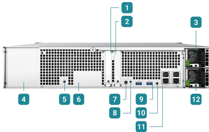
Figure 2-6 XN5112RE Rear Panel Layout
